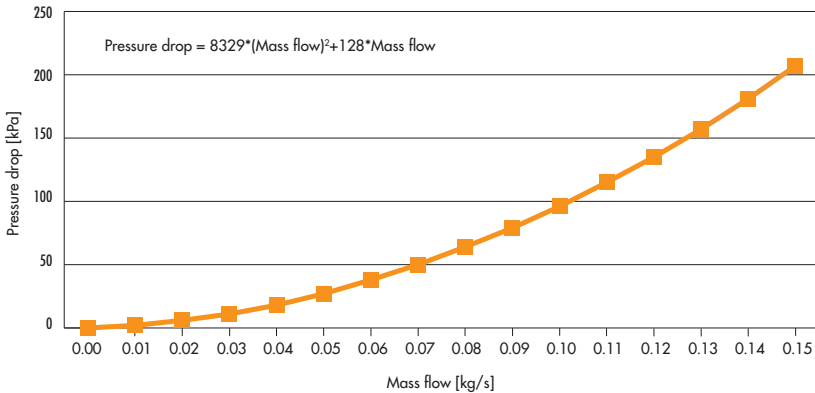
Figure 3. Pressure drop is an optional test in the standard. Different heat transfer fluids give different curves
