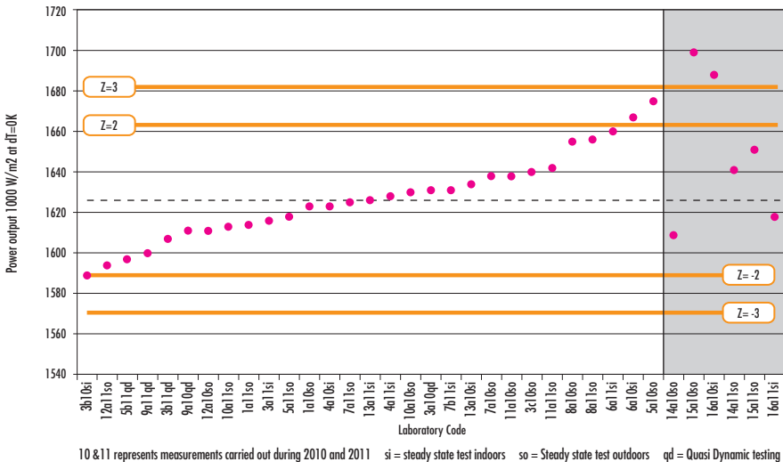
10 & 11 represents measurements carried out during 2010 and 2011 si = steady state test indoors so = Steady state test outdoors qd = Quasi Dynamic testing
